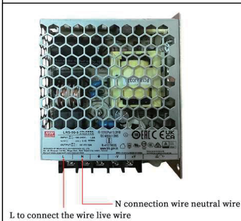
Electrical connection instructions
