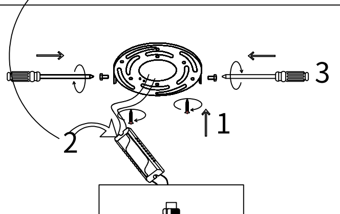
Installation instructions for ceiling tray
