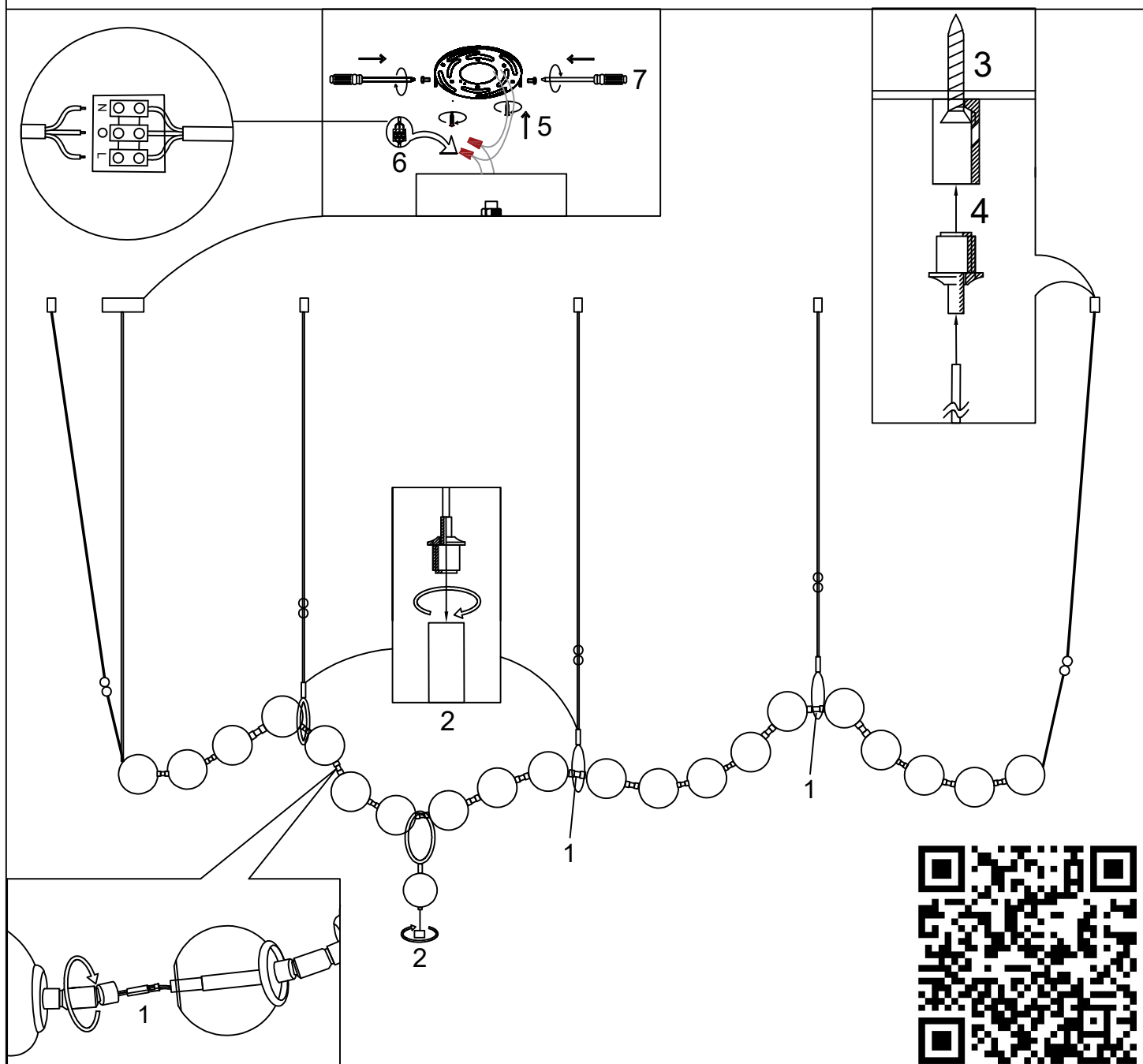
Diagram of Connection at Segments
